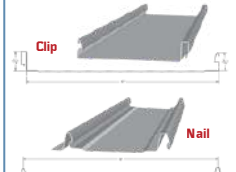
Standing Seam (Clip or Nail)
